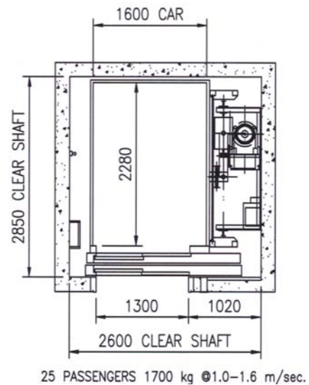
2-SPEED SIDE OPENING DOORS
