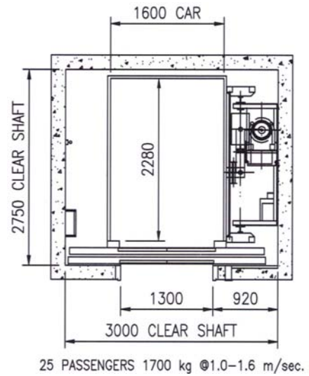
CENTRE-PARTING DOORS
