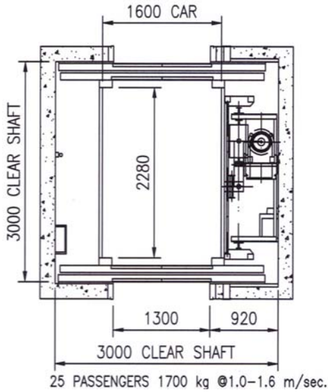
CENTRE-PARTING DOORS
