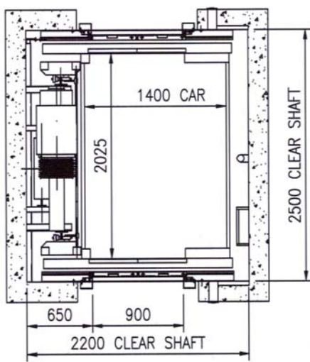
16 PASSENGERS 1088 kg @1.0–1.6 m/sec.
