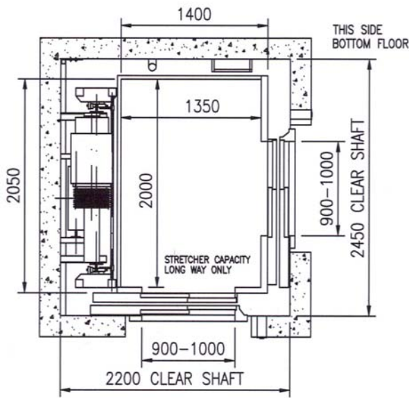
16 PASSENGERS 1088 kg @ 1.0-1.6 m/sec.
