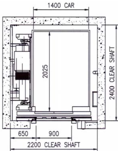
16 PASSENGERS 1088 kg @1.0–1.6 m/sec.
