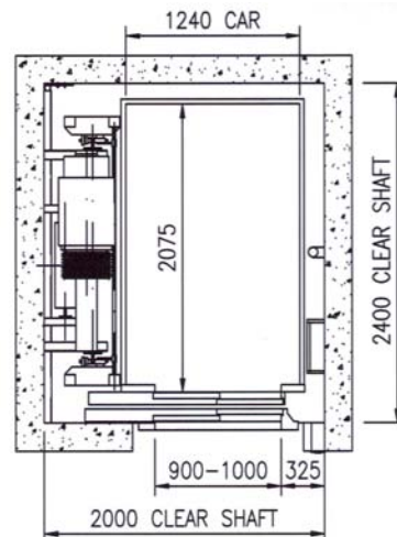
16 PASSENGERS 1088 kg @1.0–1.6 m/sec.
