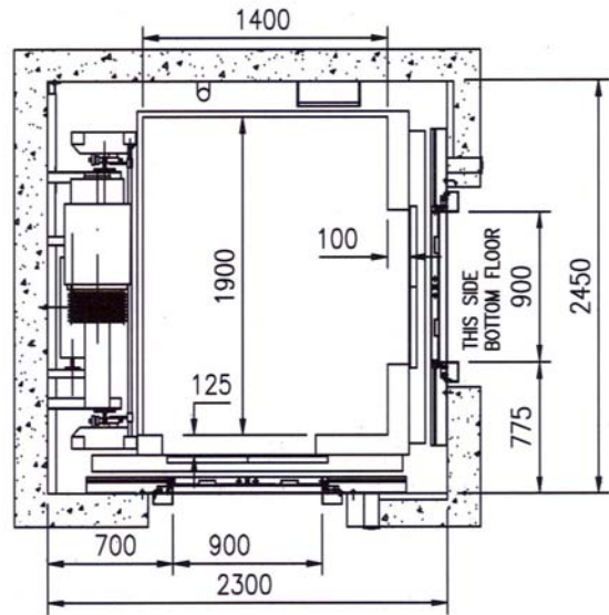
16 PASSENGERS 1088 kg @ 1.0-1.6 m/sec. STRETCHER CAPACITY ONE SIDE ONLY
